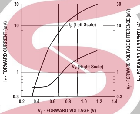
Figure 5. Typical V_f Match, Series Pairs and Quads at Mixer Bias Levels.
