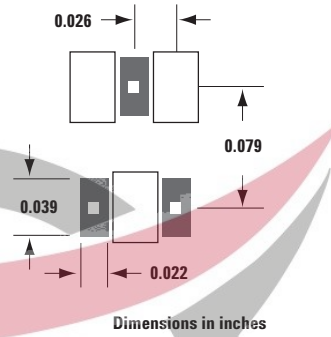
Figure 26. Recommended PCB Pad Layout for Avago's SC70 3L/SOT-323 Products.
